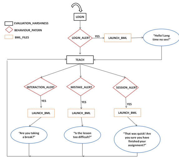
Figure 4: Evaluation FSM Example.
