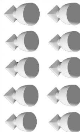
Figure 3: Left: Exact Normals. Right: Approximated Normals (weighted by Area). Resolutions of tessellations are from top to bottom: 40K, 32K, 21K, 9K and 1.6K vertices.
