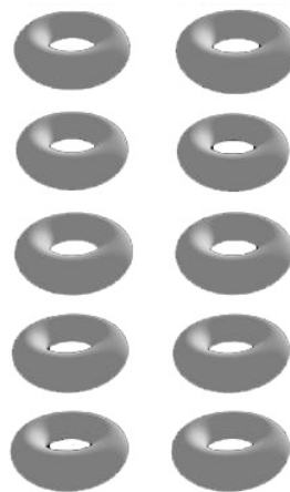
Figure 2: Left: Exact Normals. Right: Approximated Normals (weighted by Area). Resolutions of tessellations are from top to bottom: 40K, 32K, 21K, 9K and 1.6K vertices.
