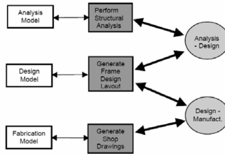
Fig. 1. Simplified process model identifying the various CIS/2 views and major exchanges, supported by high-level conformance classes [3]
