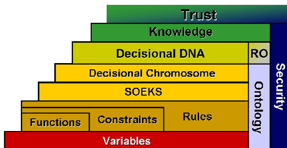
Figure 3: Decisional Trust
