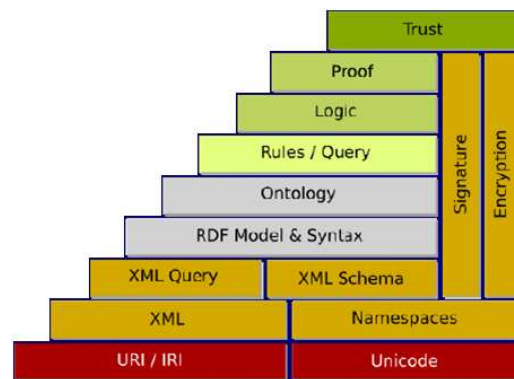
Figure 2: Semantic Web [2]
