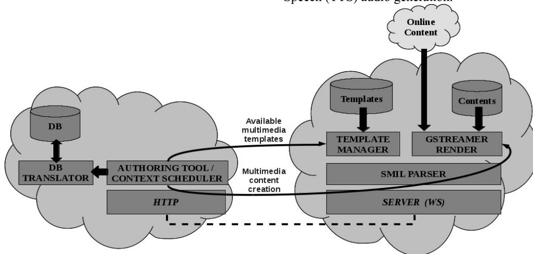
Figure 2. Architecture for dynamic multimedia creation.
