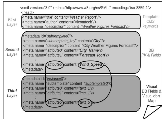
Figure 1. Semantic data for dynamic performance.
